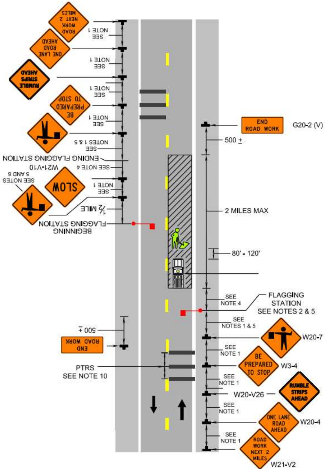
FIGURE 2 – TYPICAL INSTALLATION ON A NON-STATIONARY FLAGGING OPERATION
